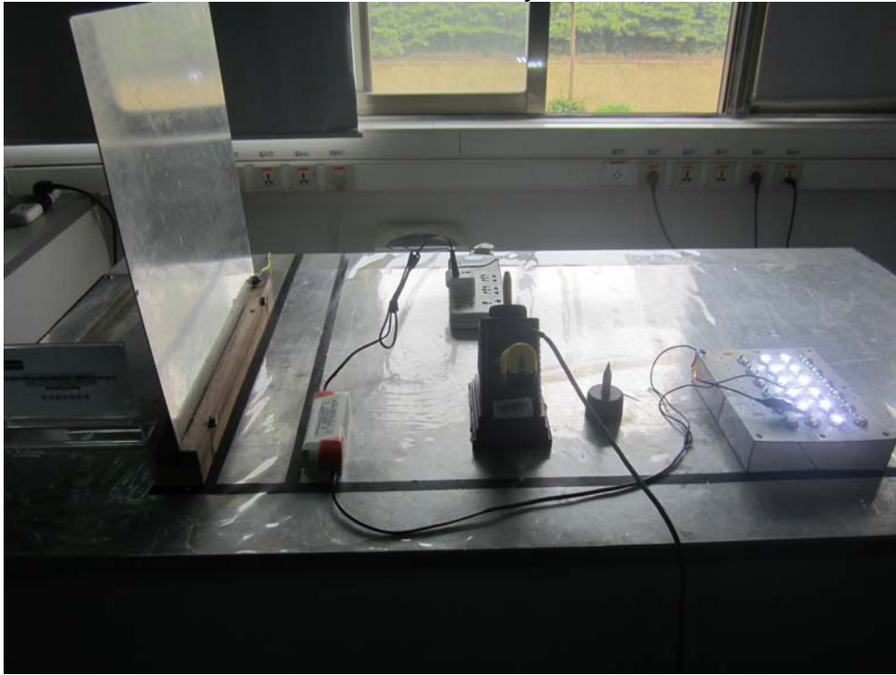
EFT/DIP Immunity
